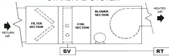
Model HS STANDARD SYSTEM
